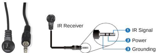
IR RECEIVER
