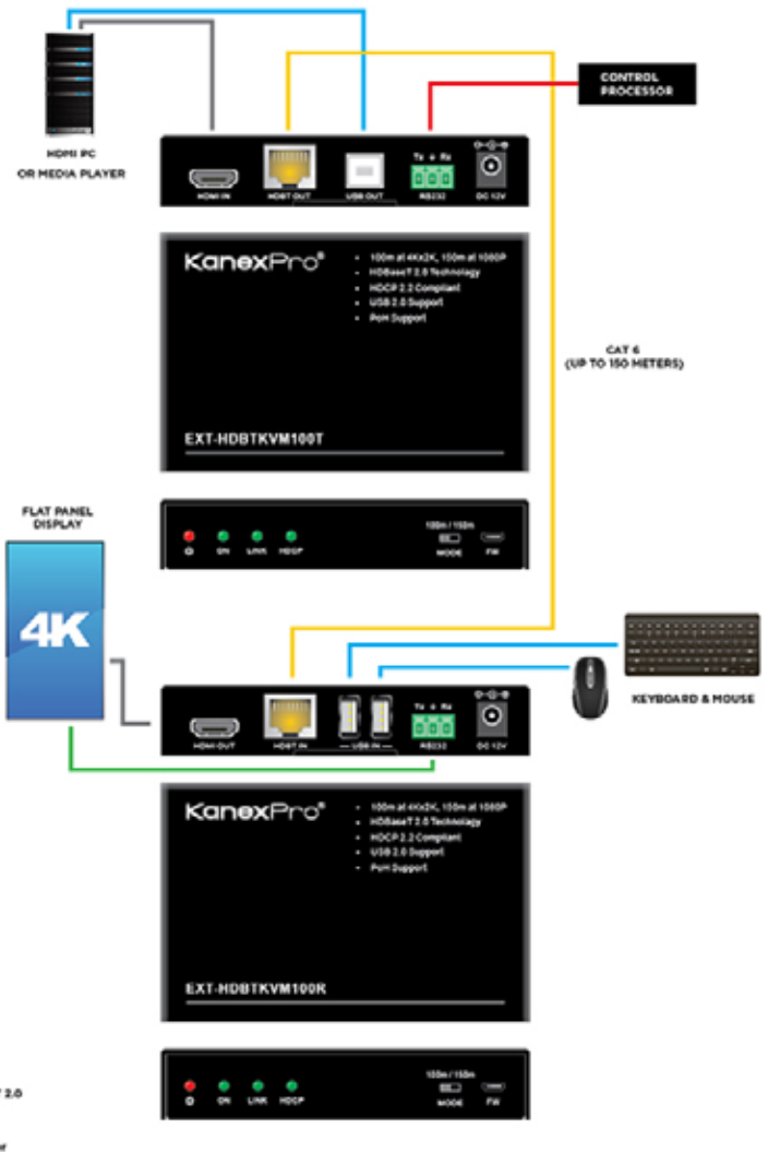
APPLICATION DIAGRAM
